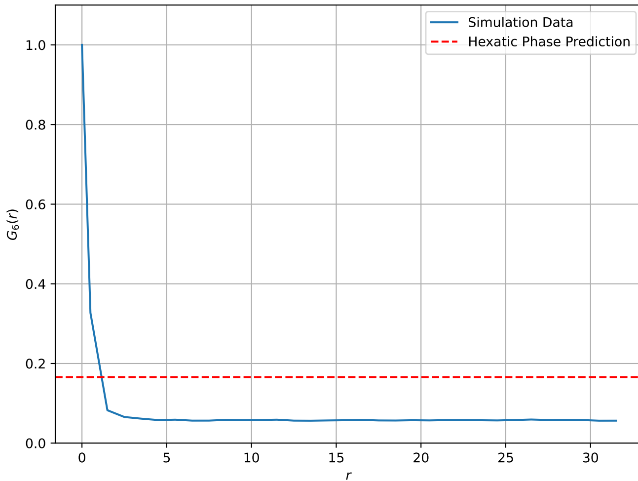
Correlation Function at T = 1.0e - 01 , L = 64
