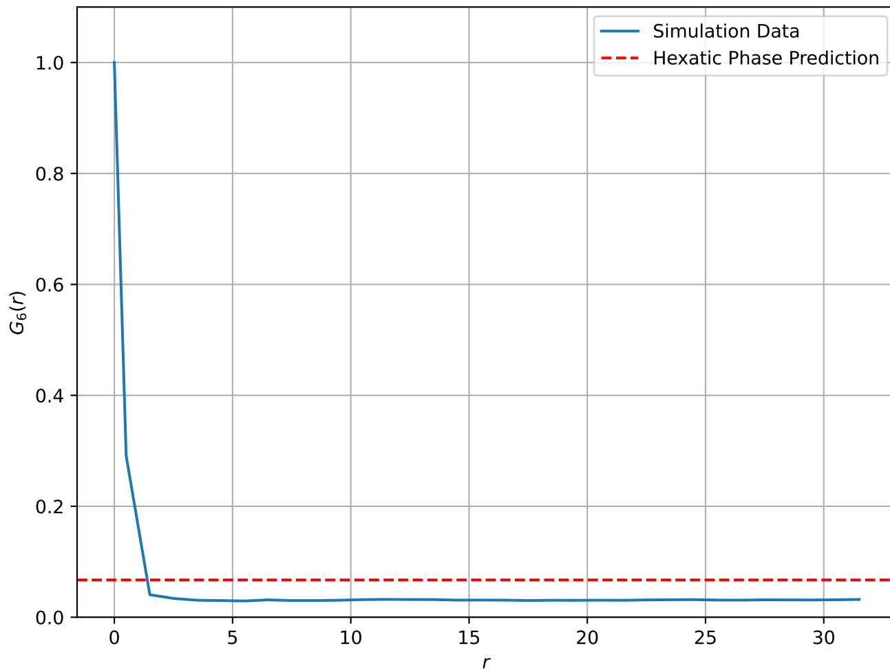
Correlation Function at T = 1.5e - 01, L = 64
