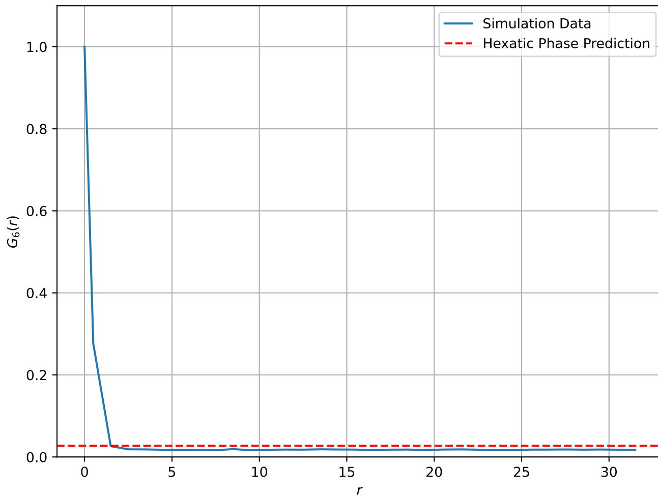
Correlation Function at T = 2.0e - 01 , L = 64
