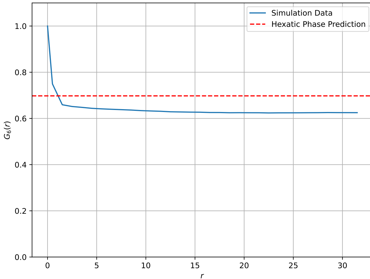
Correlation Function at T = 2.0e - 02 , L = 64
