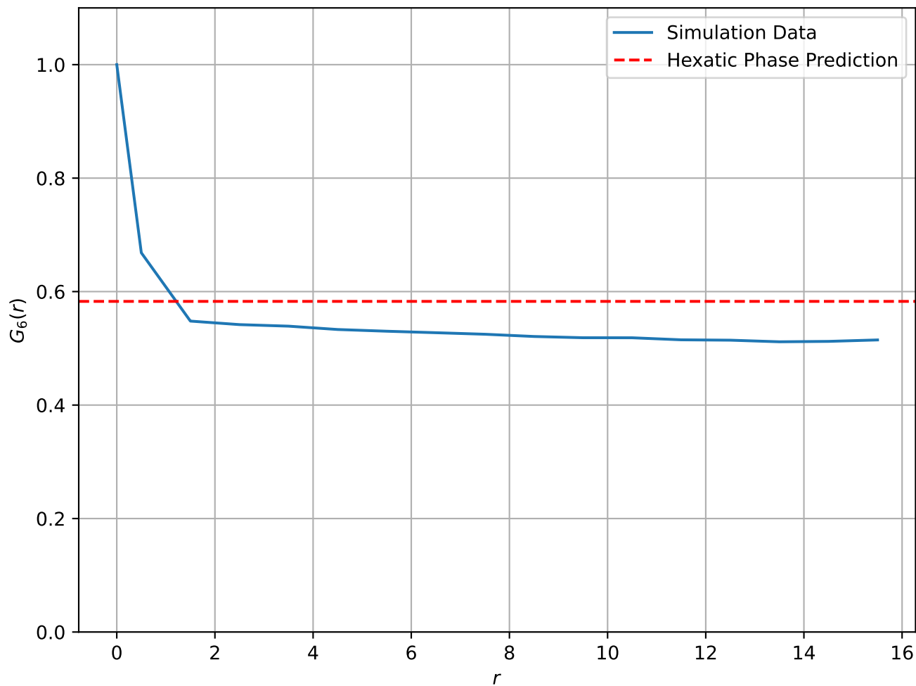
Correlation Function at T = 3.00e - 02 , L = 32
