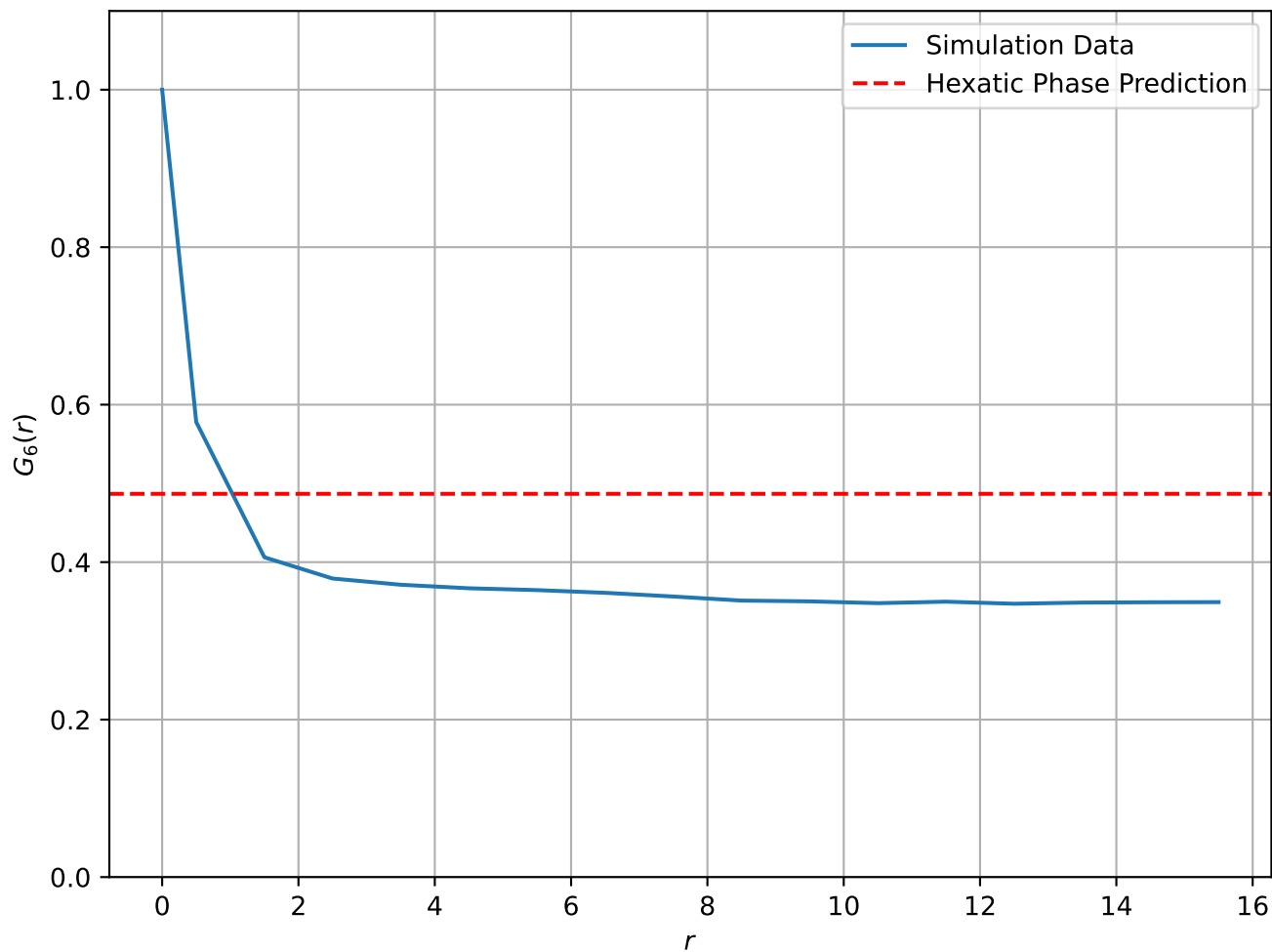
Correlation Function at T = 4.00e - 02 , L = 32
