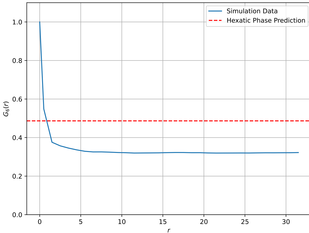
Correlation Function at T = 4.0e - 02 , L = 64
