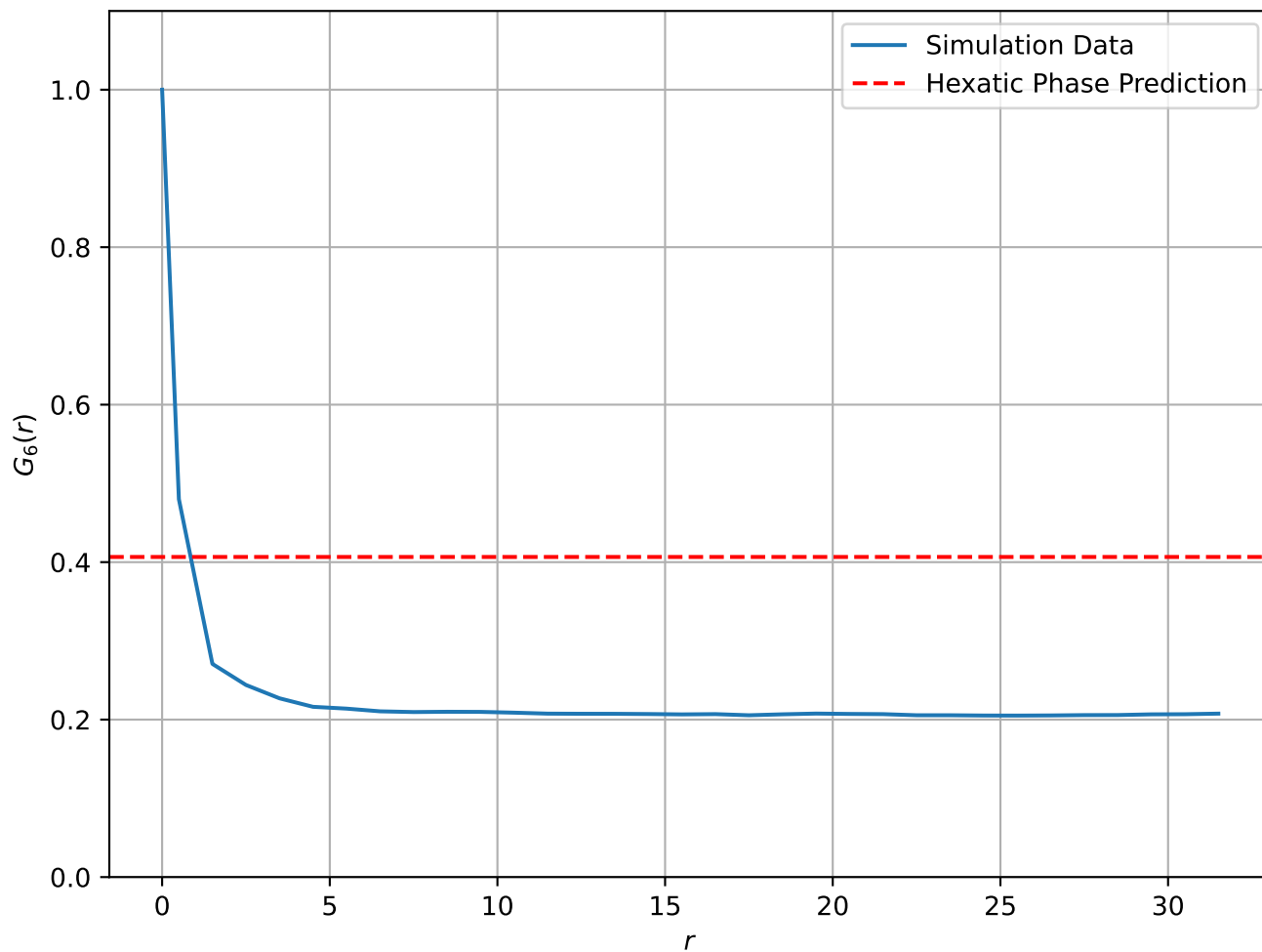
Correlation Function at T = 5.0e - 02 , L = 64
