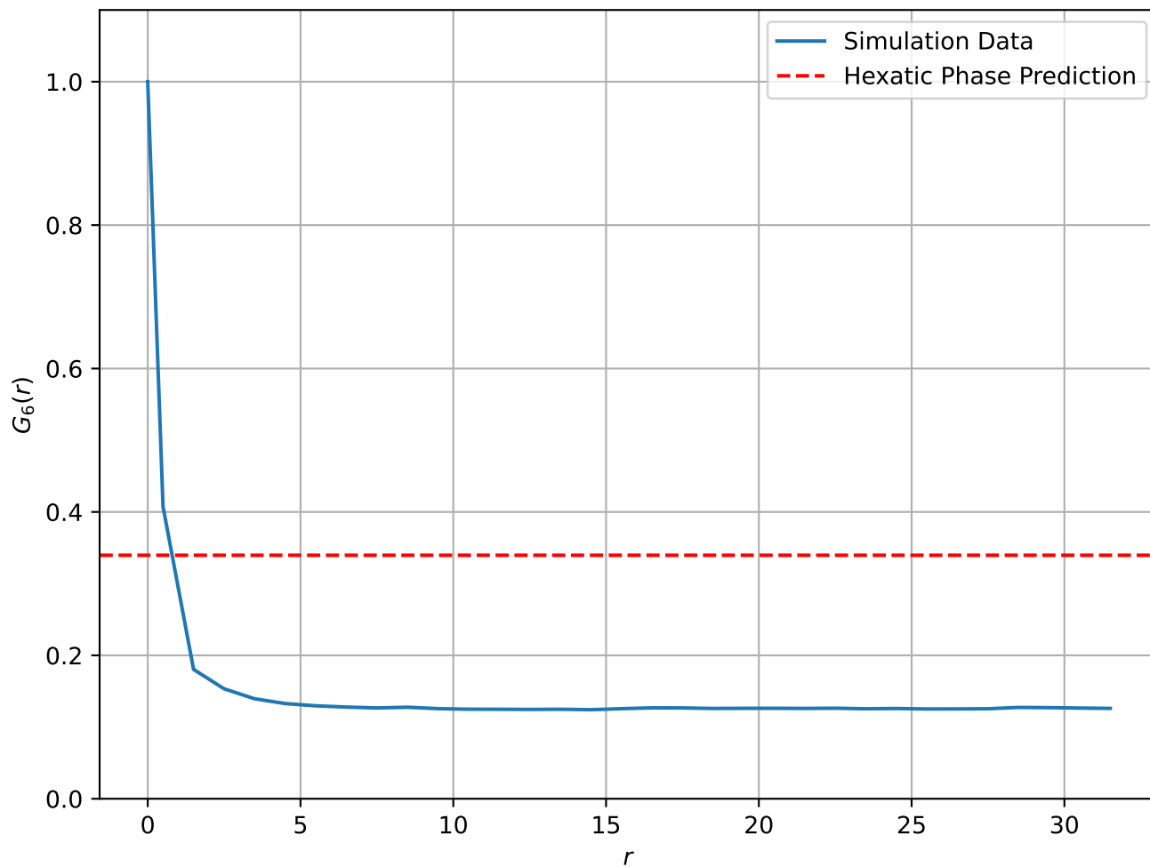
Correlation Function at T = 6.0e - 02 , L = 64
