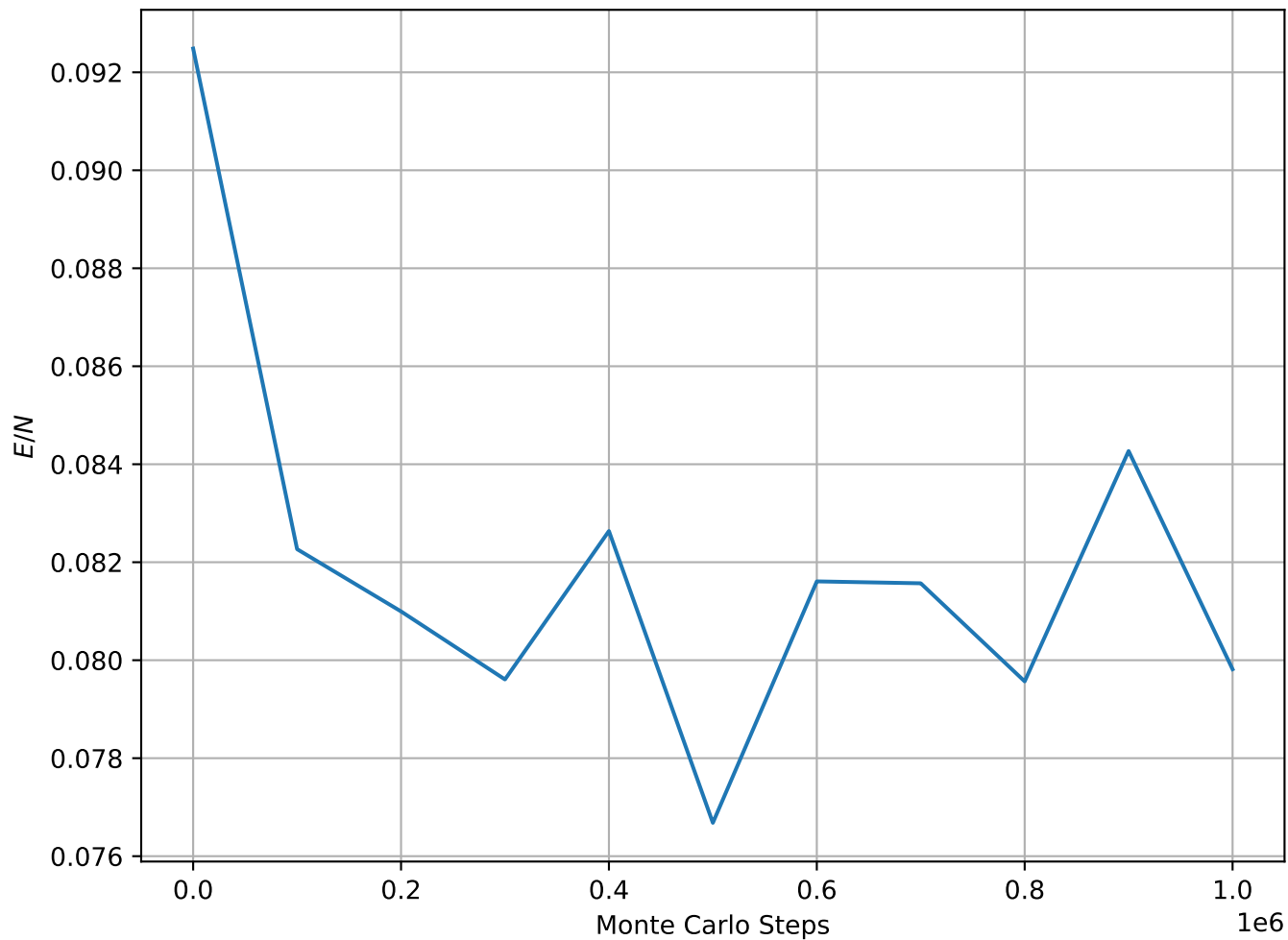
Energy per Spin at T = 1.0e - 01 , L = 64
