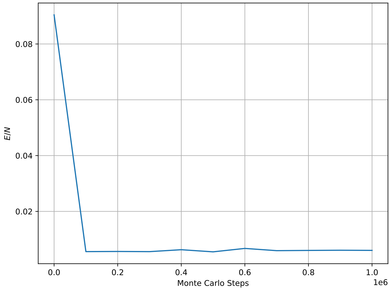
Energy per Spin at T = 1.00e - 02 , L = 32
