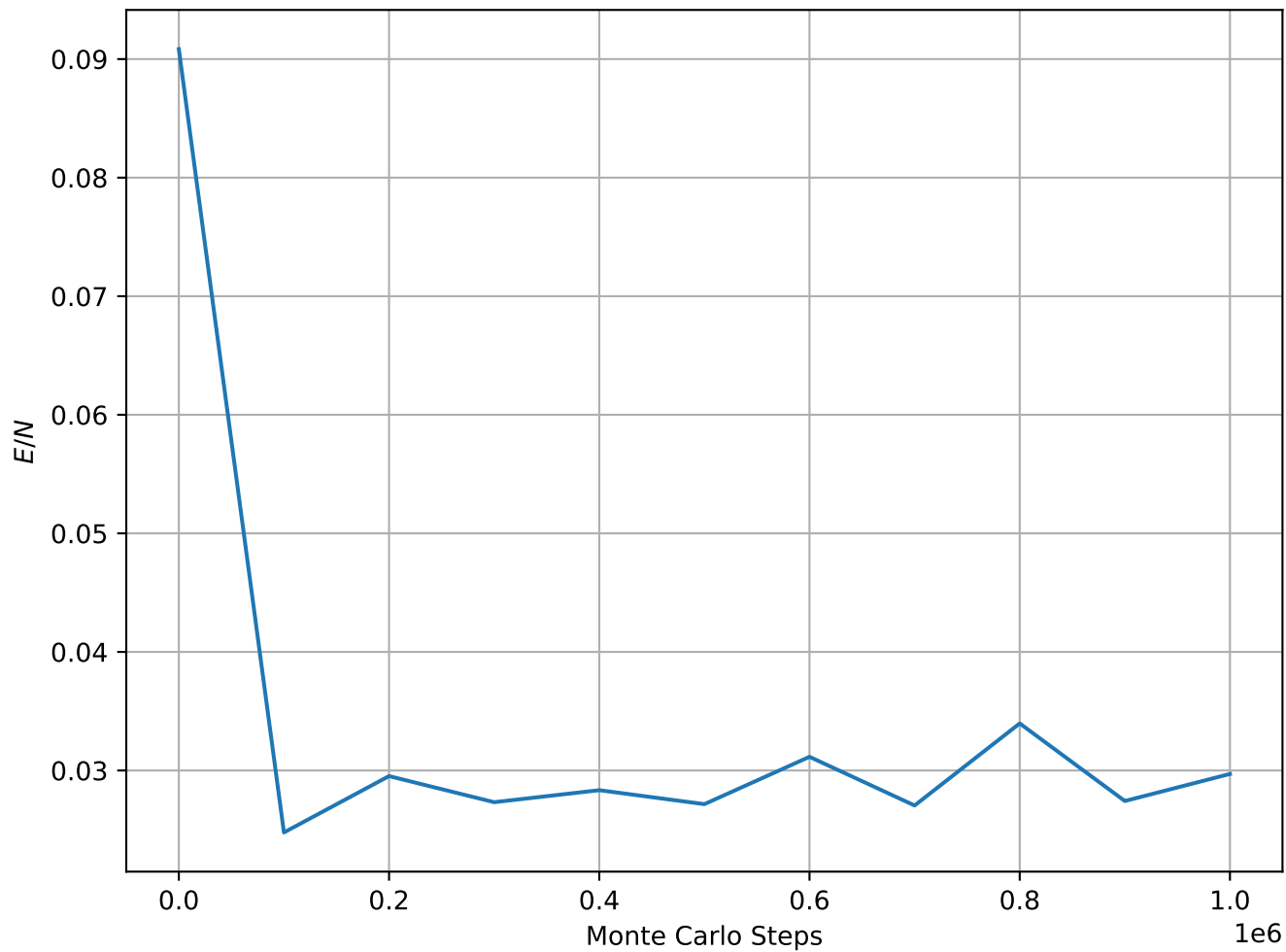
Energy per Spin at T = 4.00e - 02 , L = 32
