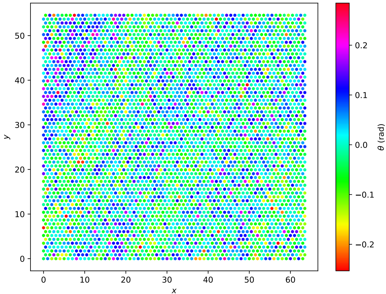
Hexagonal Lattice L=64 , T = 1.0e - 02
