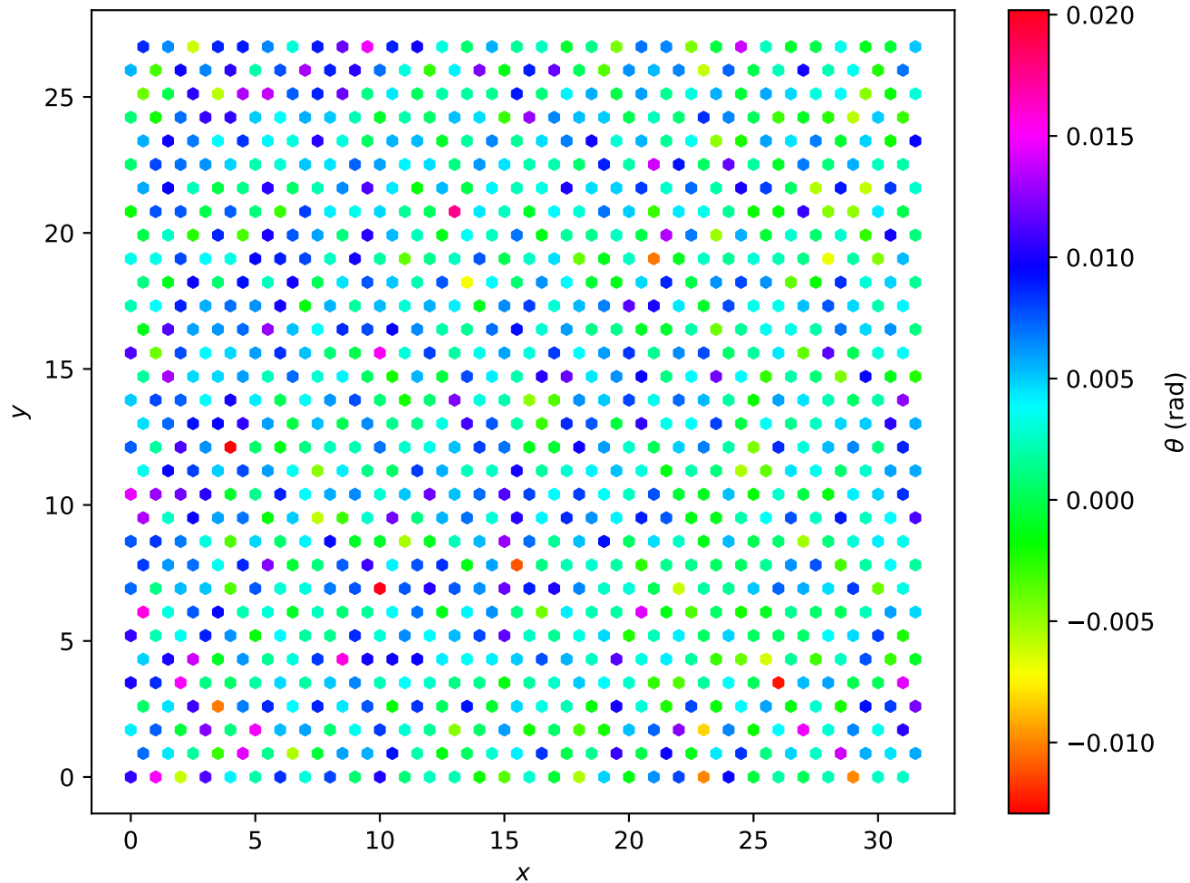
Hexagonal Lattice L=32 , T = 1.00e - 05
