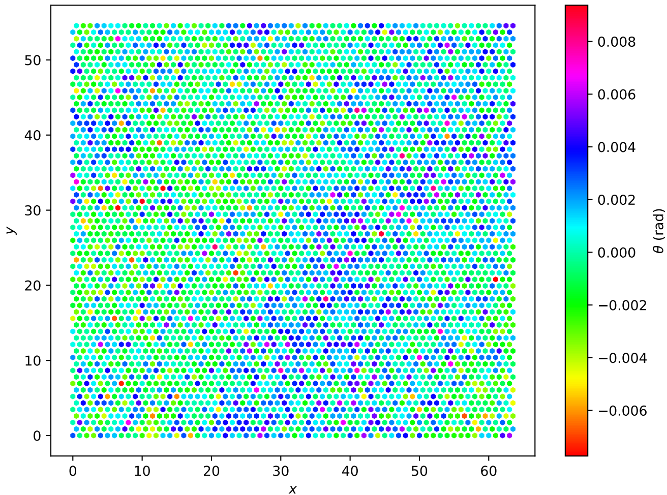
Hexagonal Lattice L=64 , T = 1.0e - 05
