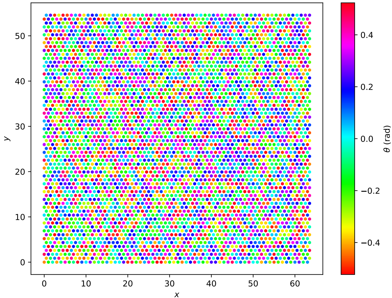
Hexagonal Lattice L=64 , T = 1.5e - 01
