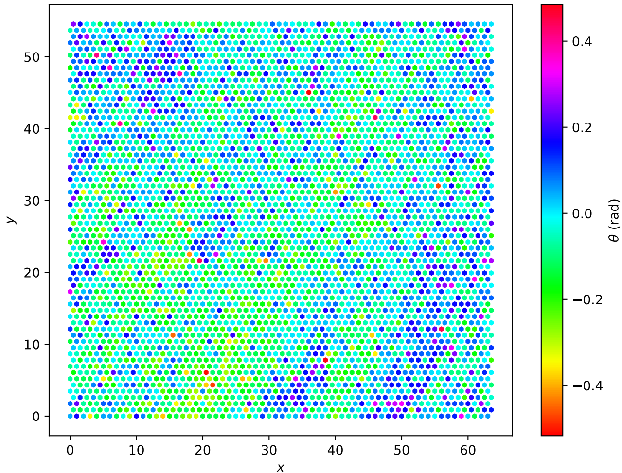
Hexagonal Lattice L=64 , T = 2.0e - 02
