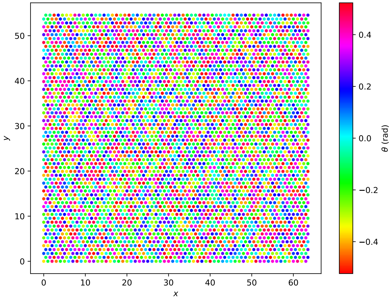
Hexagonal Lattice L=64 , T = 2.5e - 01
