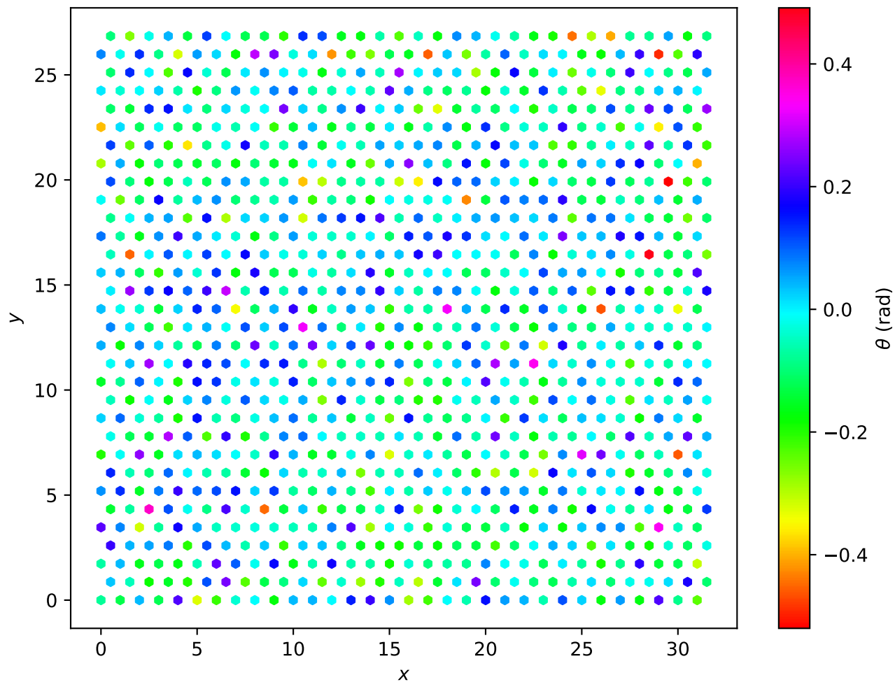
Hexagonal Lattice L=32 , T = 3.00e - 02
