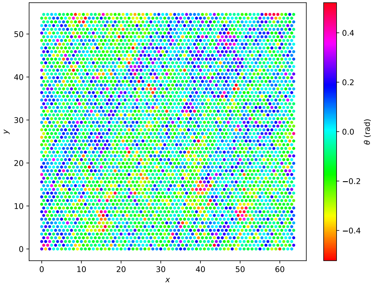
Hexagonal Lattice L=64 , T = 3.0e - 02
