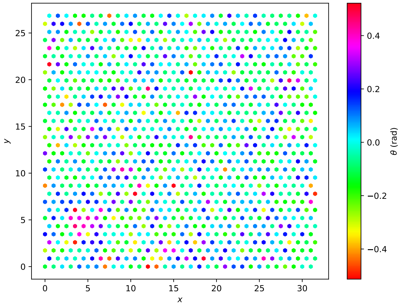
Hexagonal Lattice L=32 , T = 4.00e - 02
