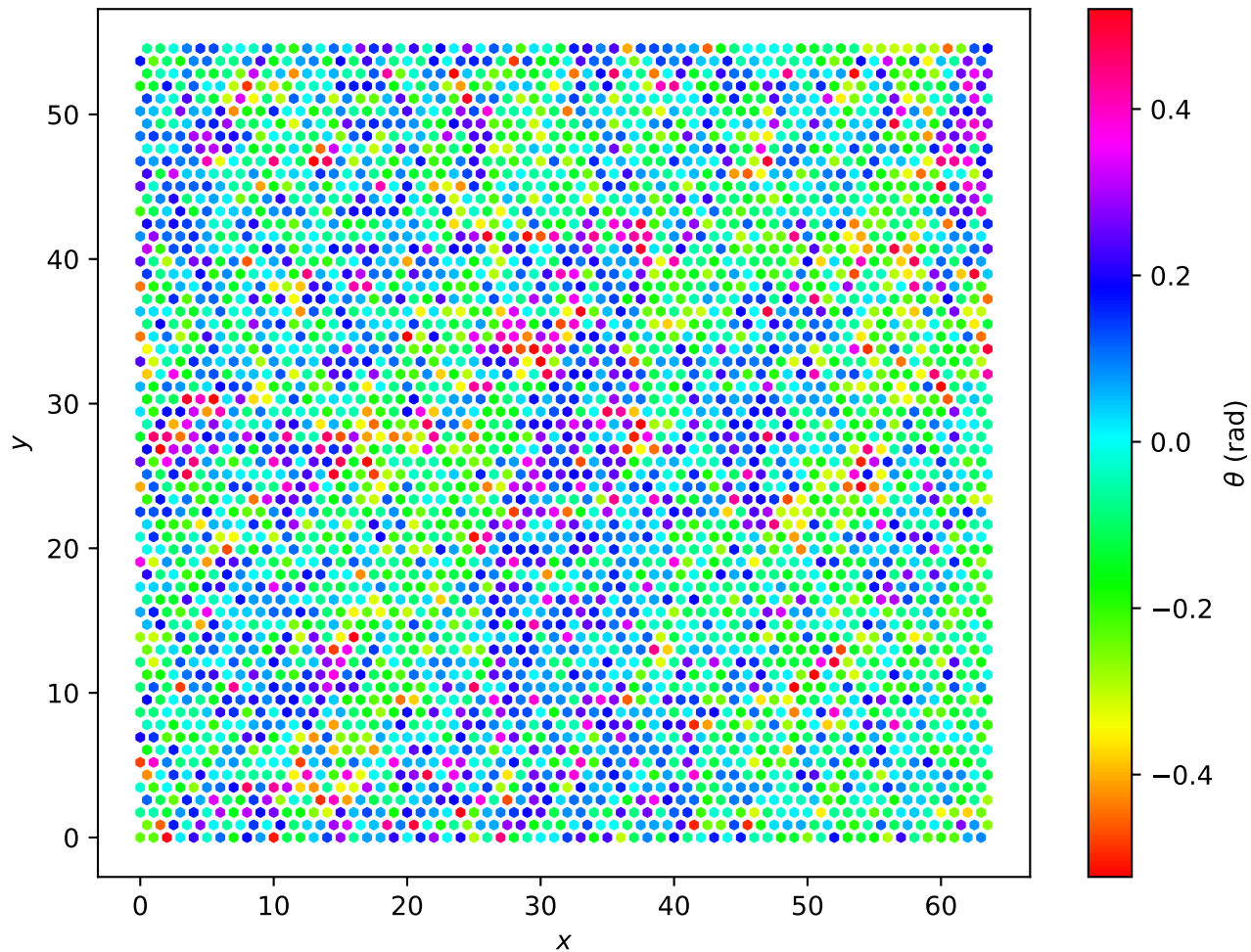
Hexagonal Lattice L=64 , T = 4.0e - 02
