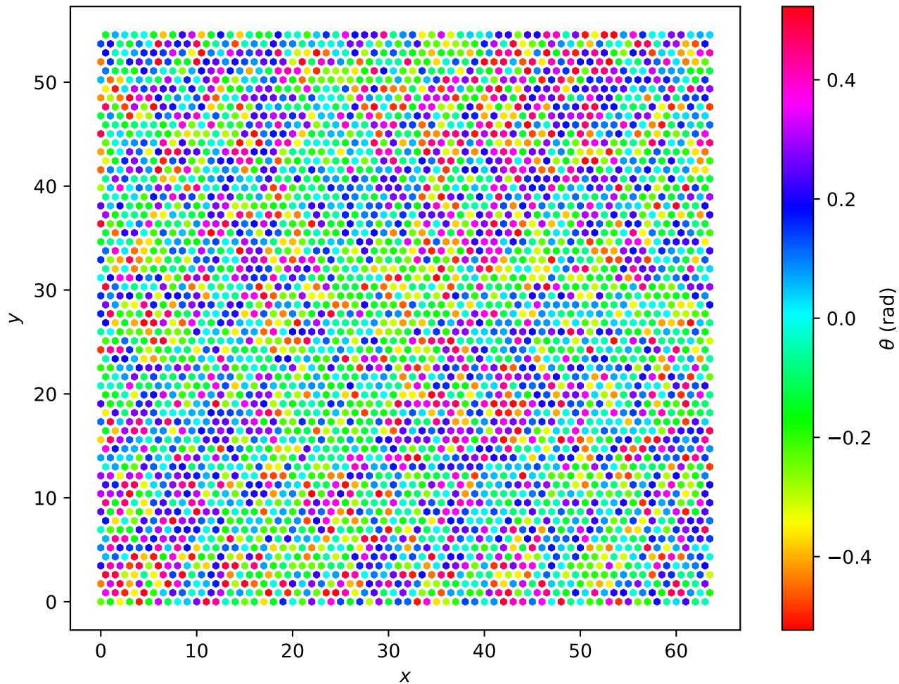
Hexagonal Lattice L=64 , T = 6.0e - 02
