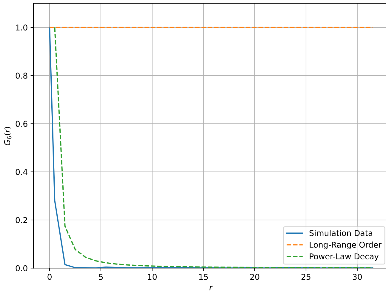
Correlation Function at T = 1.0e + 01
