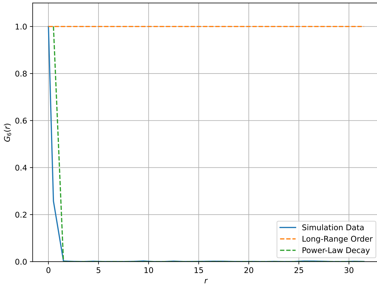
Correlation Function at T = 1.0e + 05
