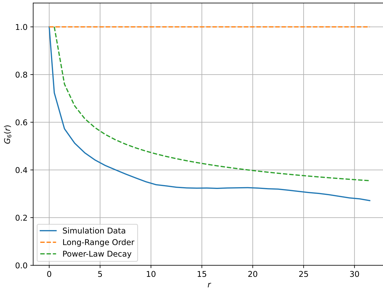
Correlation Function at T = 1.6e + 00
