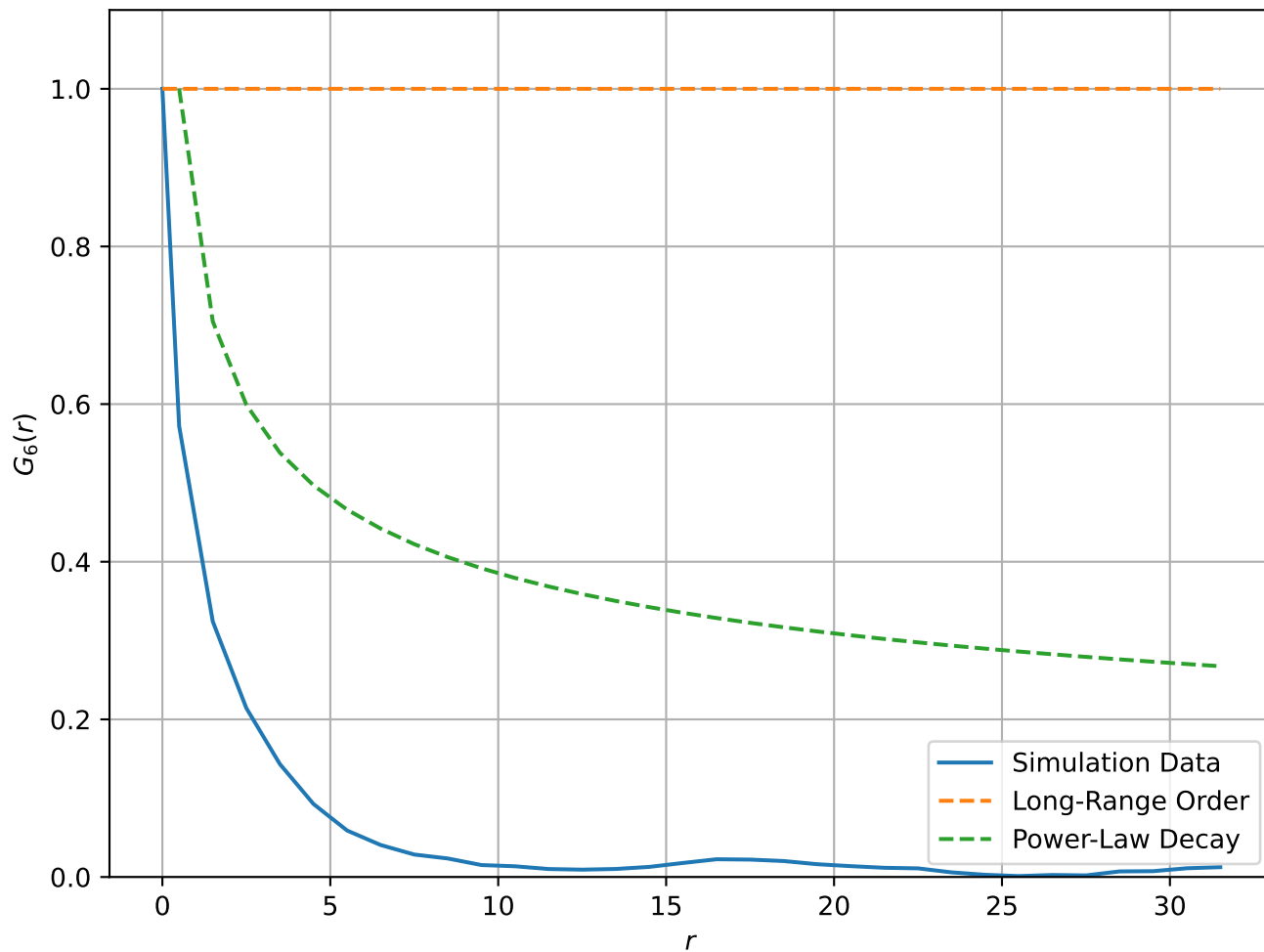
Correlation Function at T = 2.0e + 00
