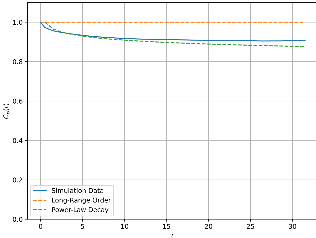
Correlation Function at T = 2.0e - 01
