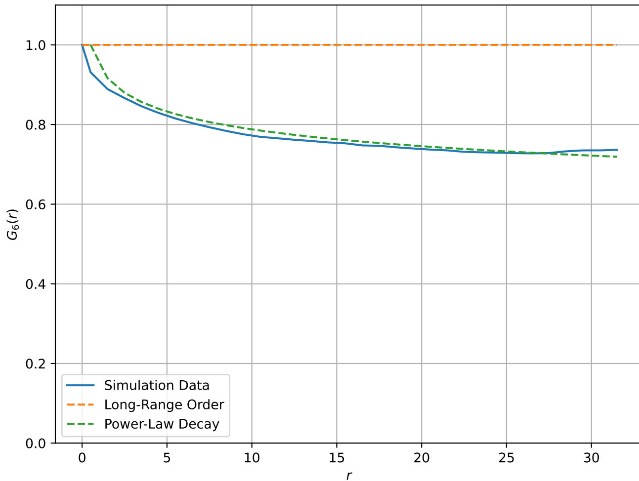
Correlation Function at T = 5.0e - 01
