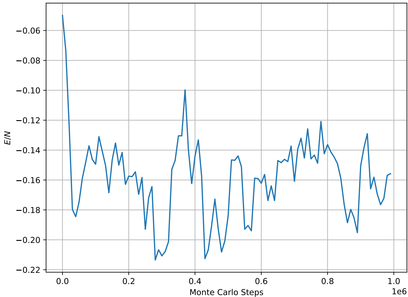
Energy per Spin at T = 1.0e + 01
