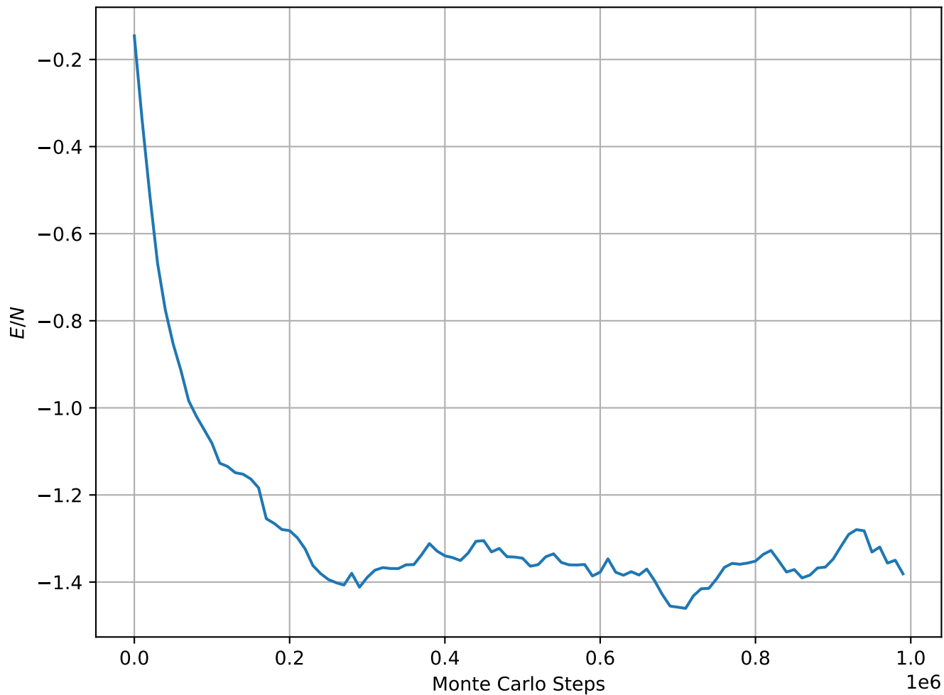
Energy per Spin at T = 2.0e + 00
