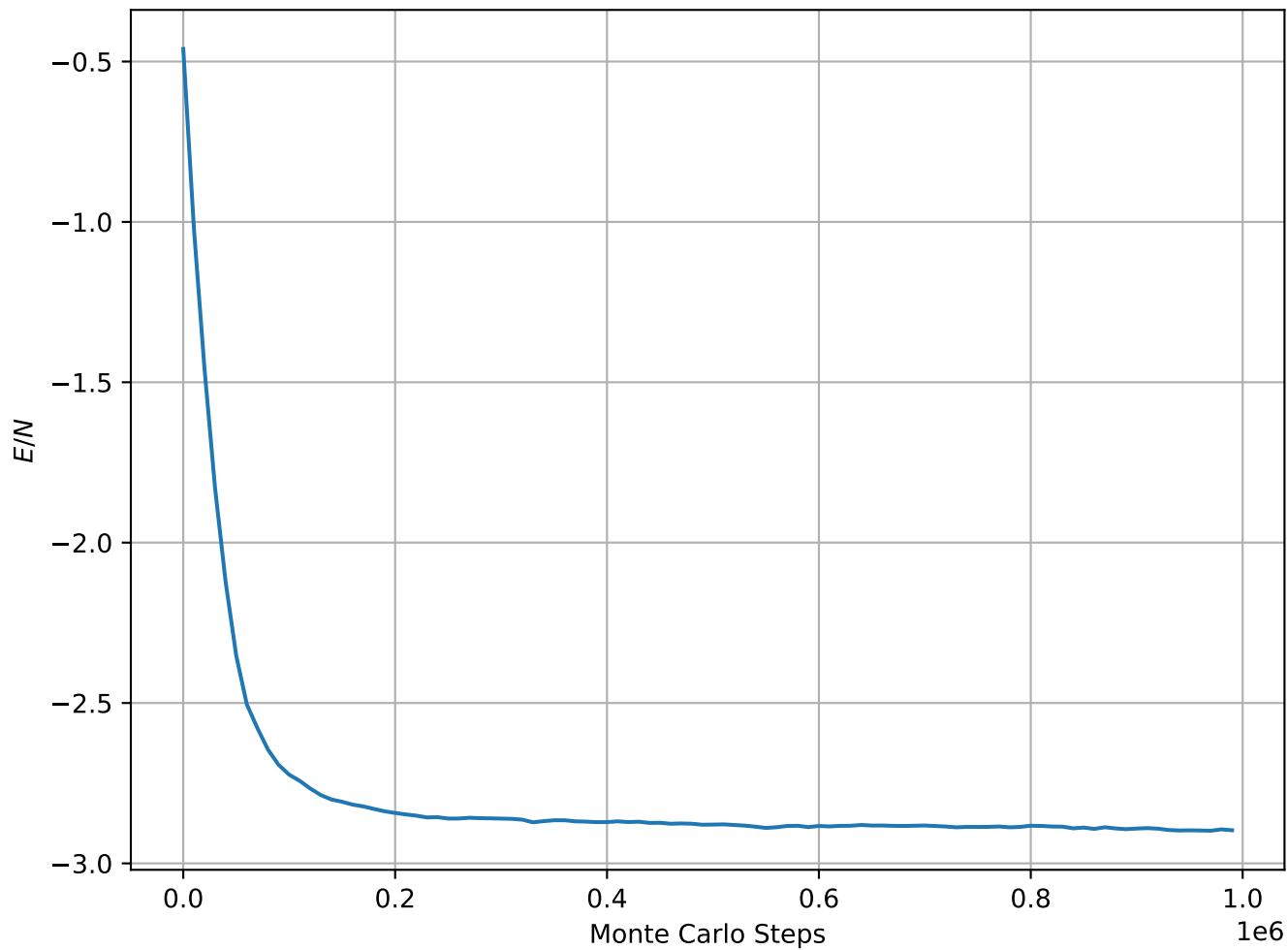
Energy per Spin at T = 2.0e - 01
