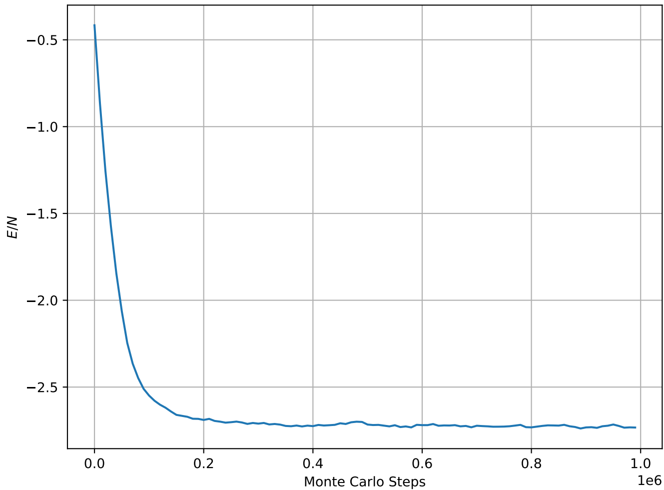
Energy per Spin at T = 5.0e - 01
