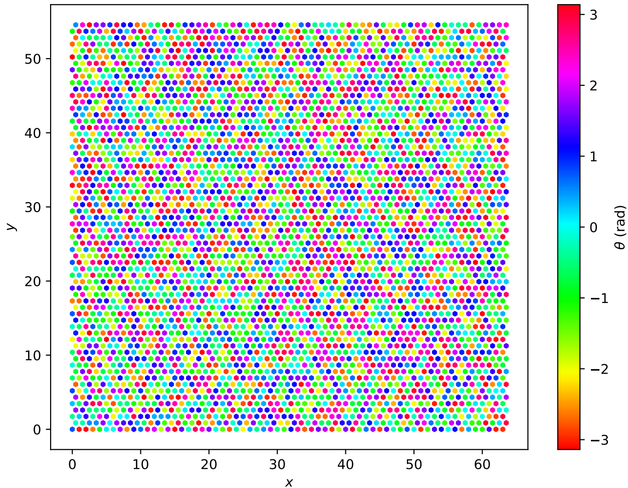
Hexagonal Lattice L=64 , T = 1.0e + 01
