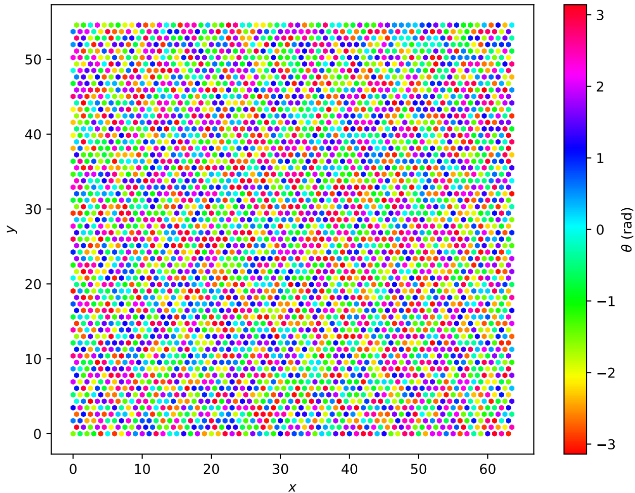
Hexagonal Lattice L=64 , T = 1.0e + 05
