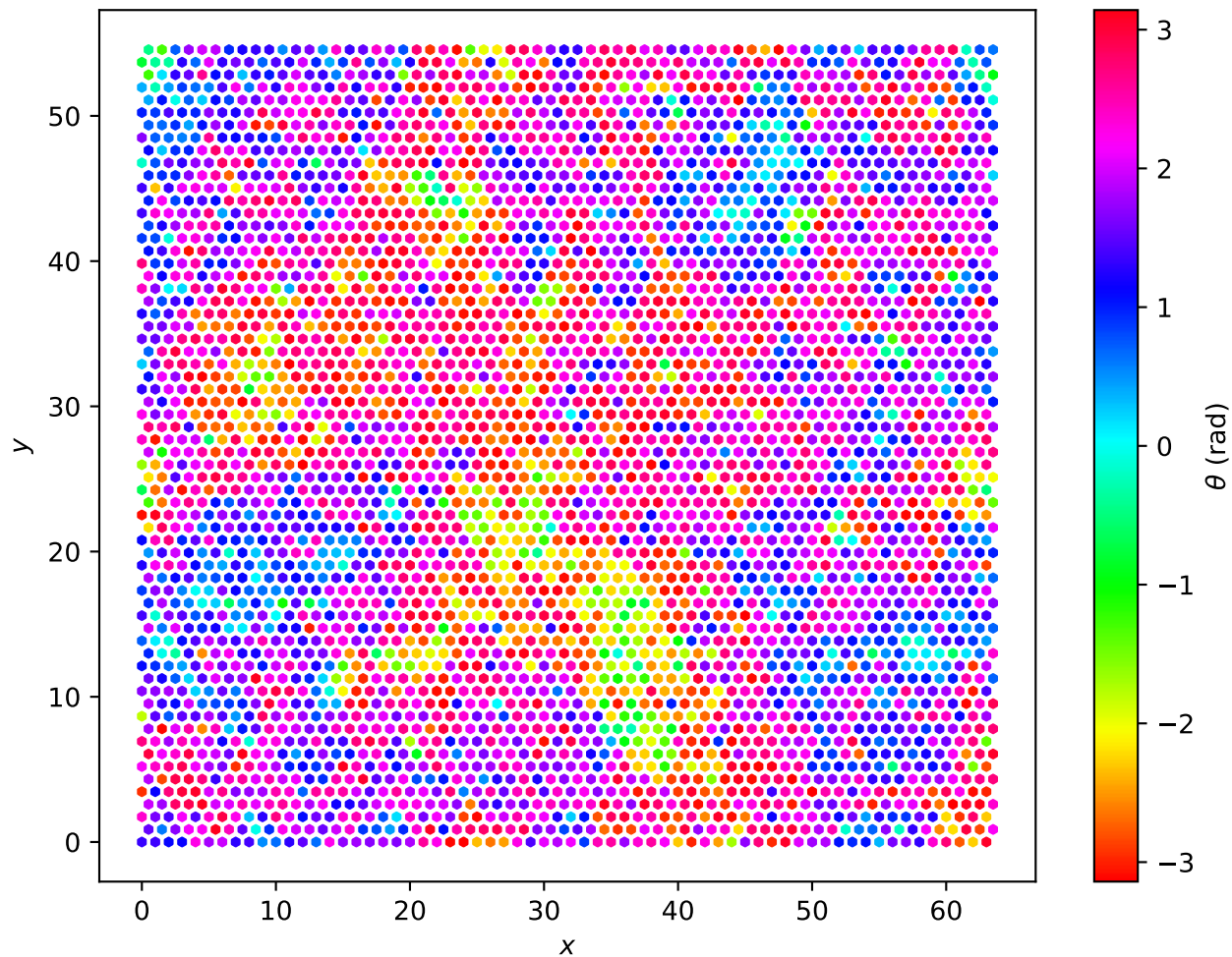
Hexagonal Lattice L=64 , T = 1.6e + 00
