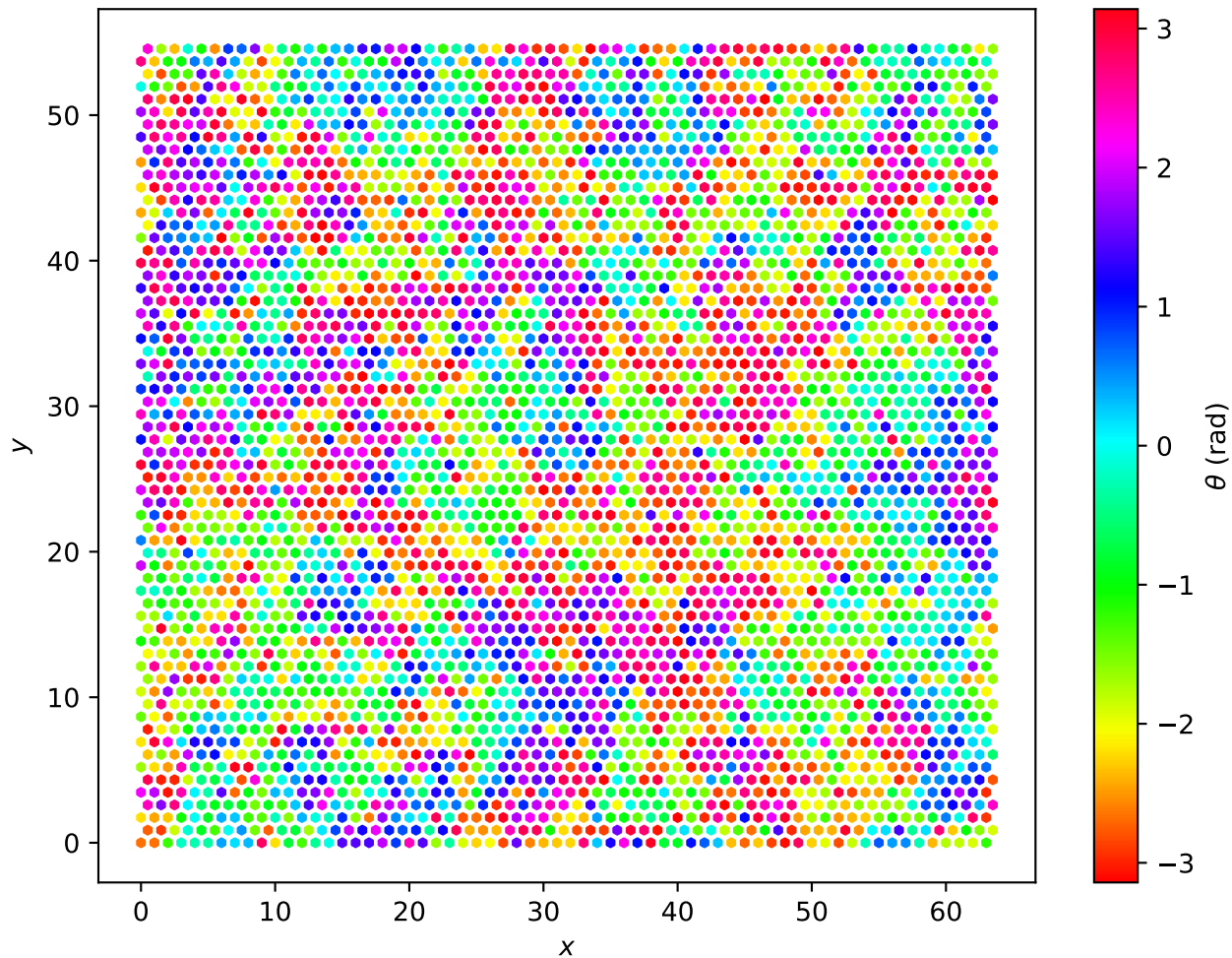
Hexagonal Lattice L=64 , T = 2.0e + 00
