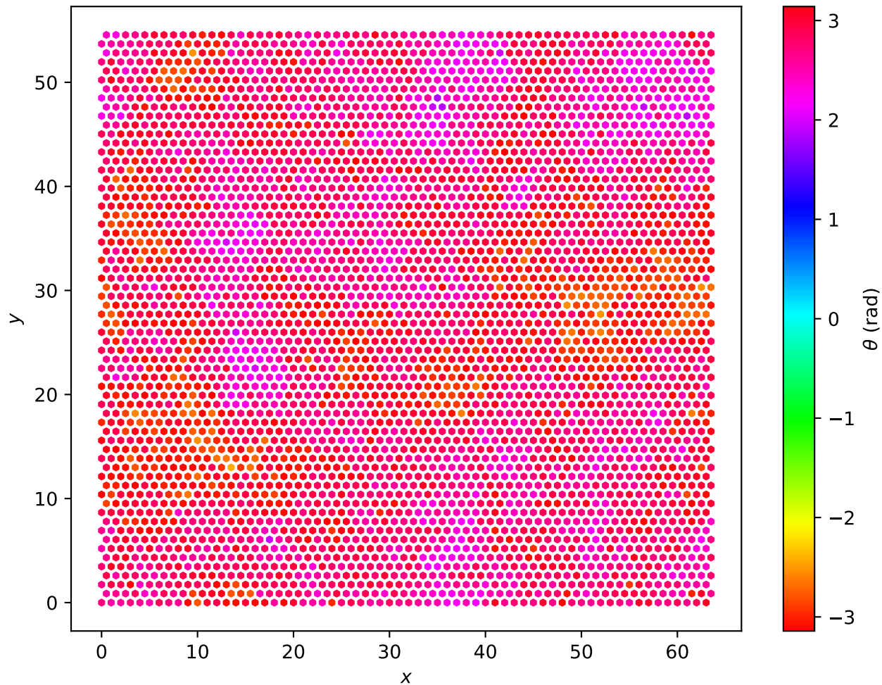
Hexagonal Lattice L=64 , T = 2.0e - 01
