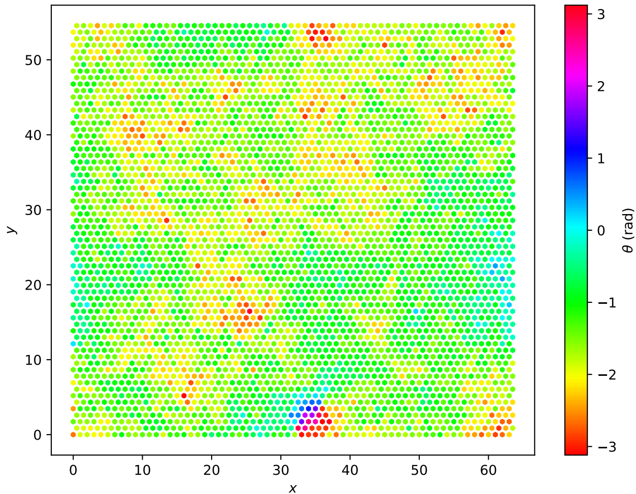
Hexagonal Lattice L=64 , T = 5.0e - 01
