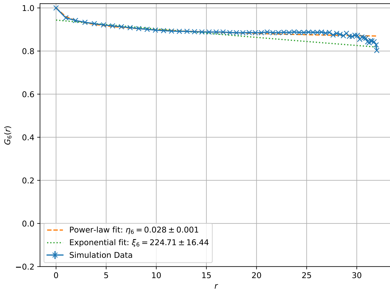
Correlation Function at T = 1.00\text{e} - 01 , L = 32
