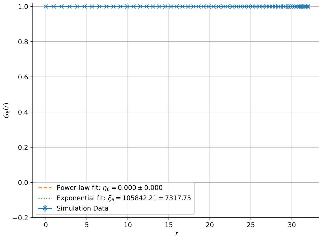
Correlation Function at T = 1.00\text{e} - 02 , L = 32
