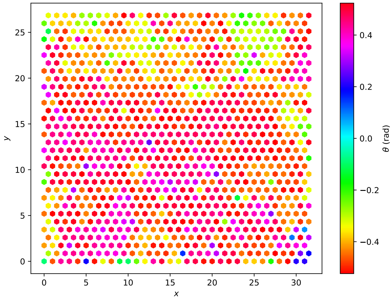
Hexagonal Lattice L=32 , T = 1.60e - 01
