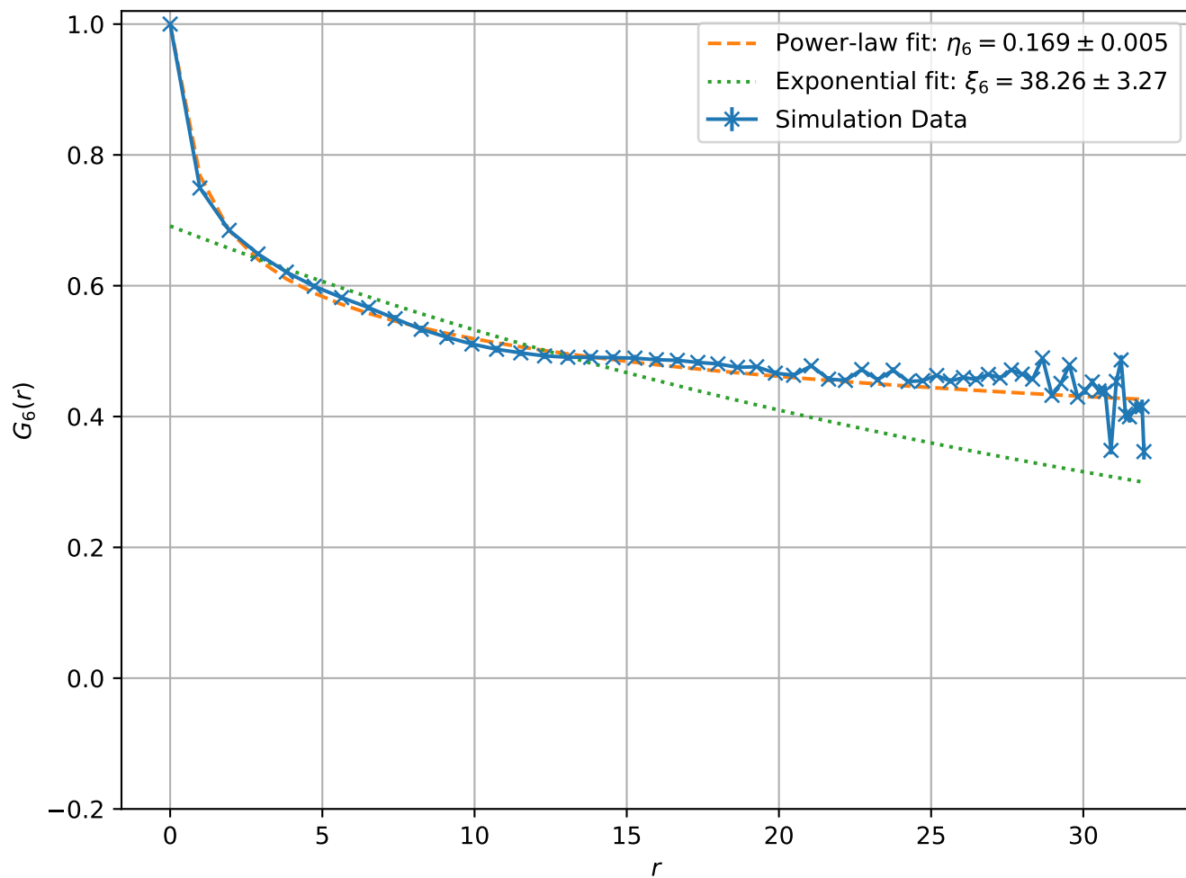
Correlation Function at T = 1.70e - 01 , L = 32
