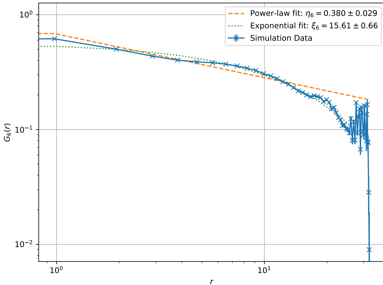
Correlation Function at T = 1.90e - 01 , L = 32 (Log-Log Scale)
