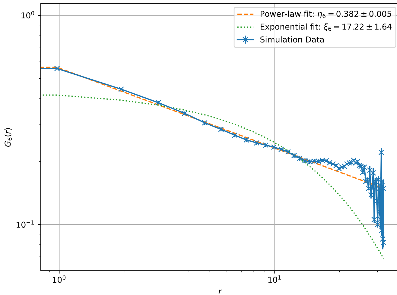
Correlation Function at T = 2.00e - 01 , L = 32 (Log-Log Scale)
