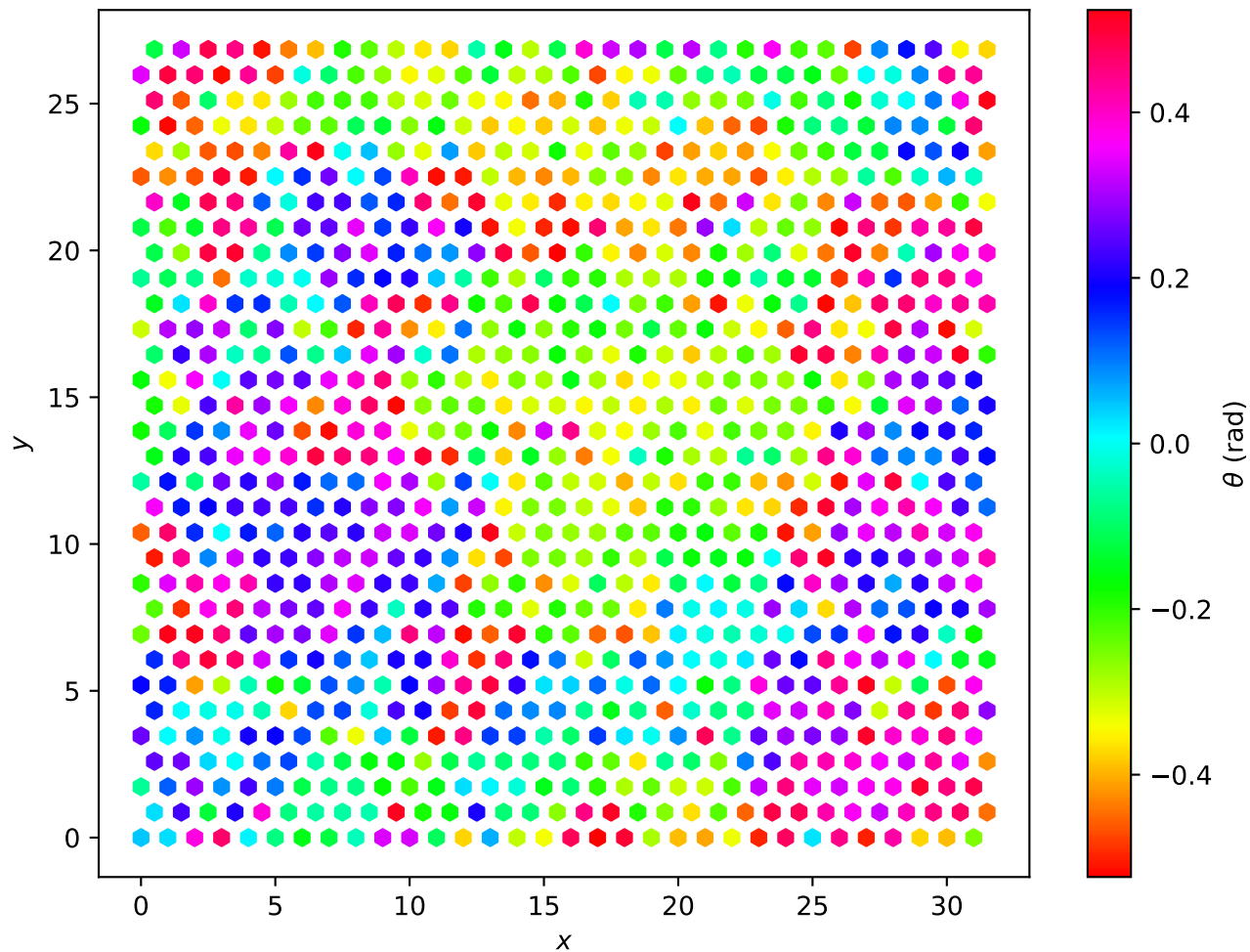
Hexagonal Lattice L=32 , T = 2.10e - 01
