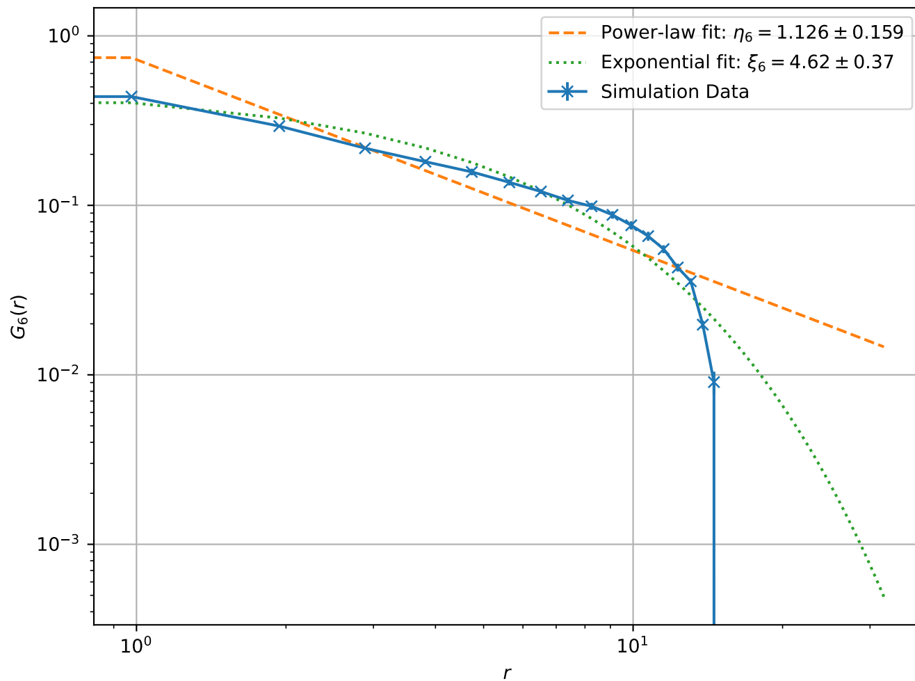
Correlation Function at T = 2.20e - 01 , L = 32 (Log-Log Scale)
