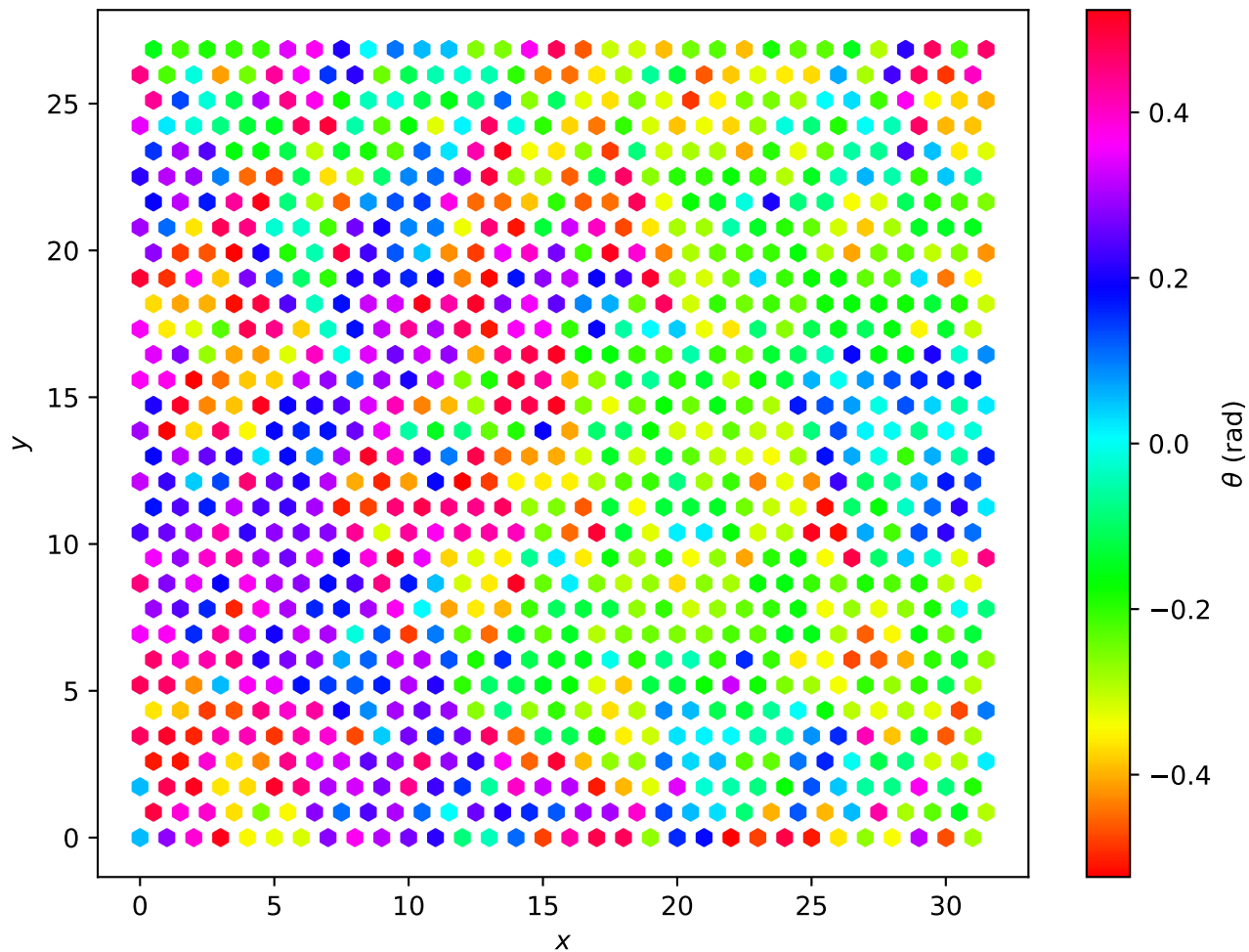
Hexagonal Lattice L=32 , T = 2.20e - 01
