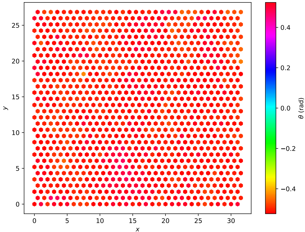
Hexagonal Lattice L=32 , T = 5.00e - 02
