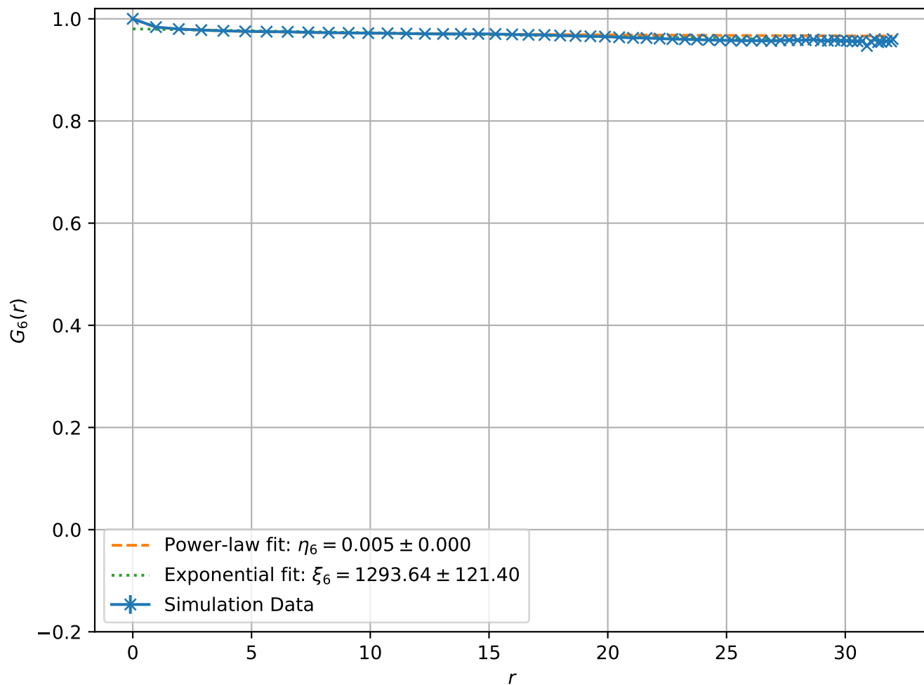
Correlation Function at T = 7.00e - 02 , L = 32
